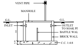
SECTION OF SEP. TANK
