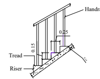
STAIRCASE DETAIL
