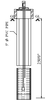
BOREWELL DETAILS
