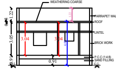
SECTION ON "AA"
