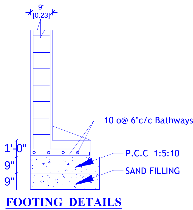
FOOTING DETAILS
