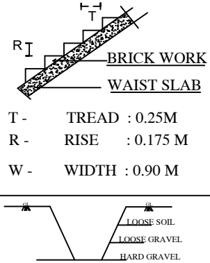
STAIRCASE DETAILS (NOT TO SCALE)
