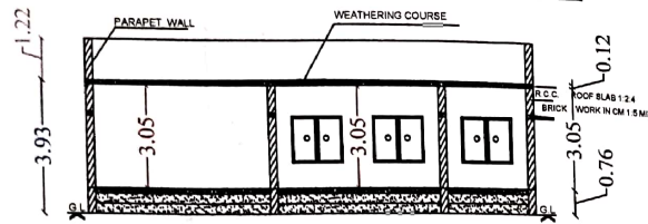
Section on-"AA"
