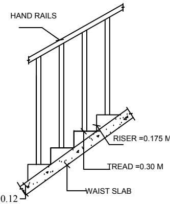
STAIR CASE DETAILS
