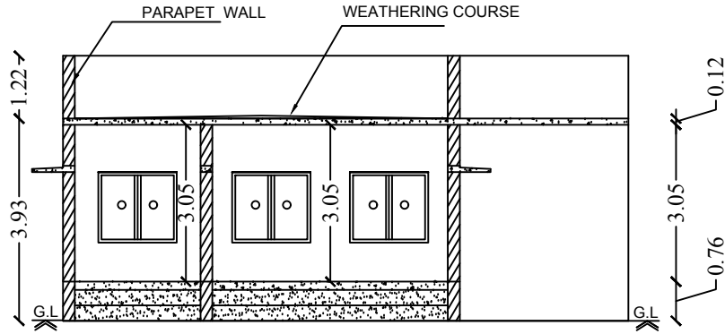
Section on-"AA"
