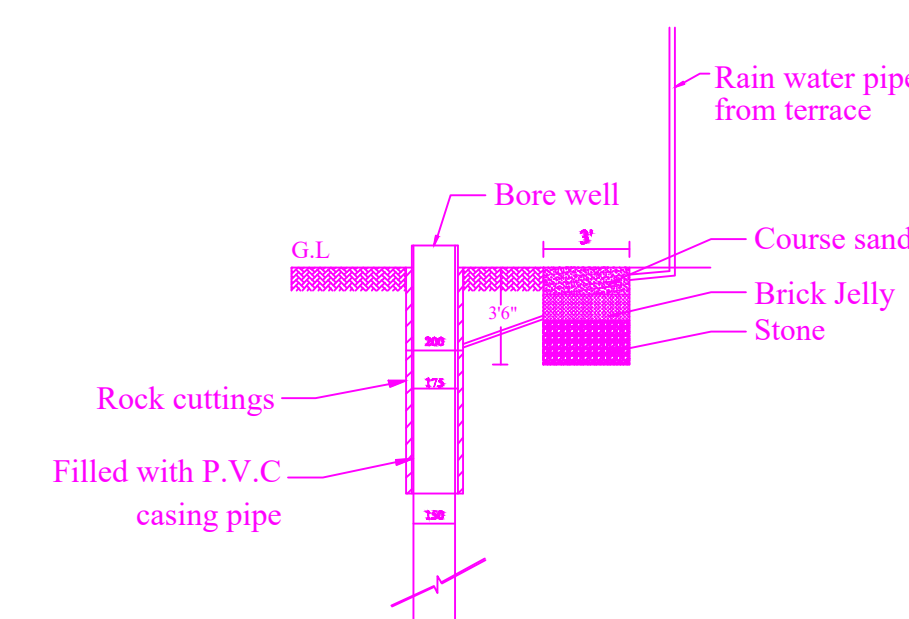
RAIN WATER HARVESTING DETAIL
