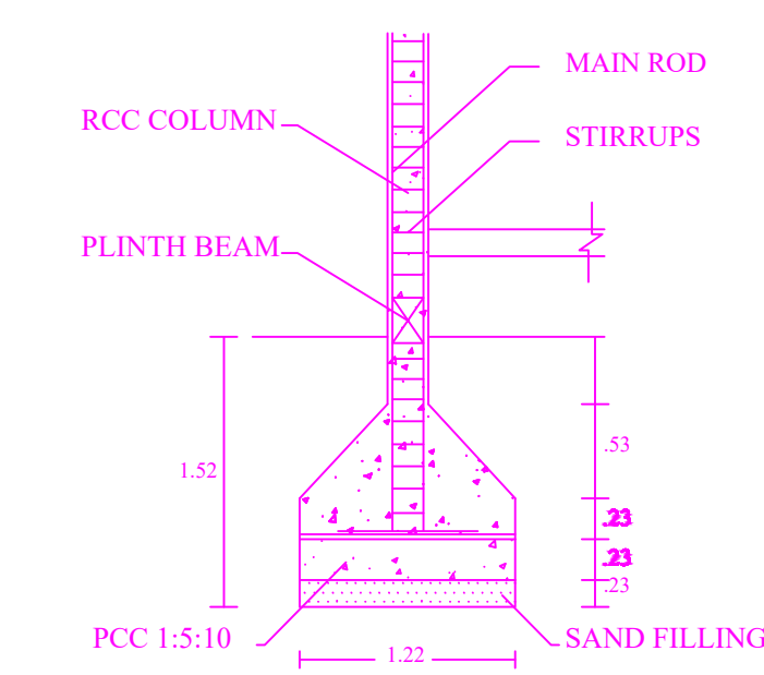
COLUMN DETAILS
