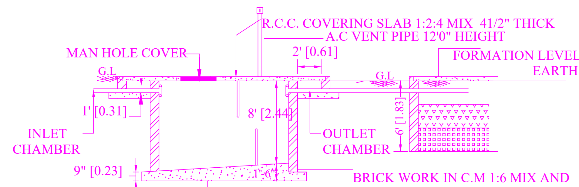
SEPTIC TANK
