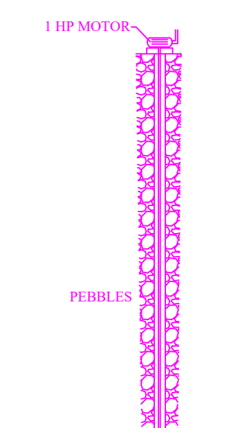
BORE WELL
