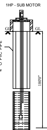
Bore Well Details
