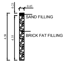
DETAILS OF RCULATION PIT
