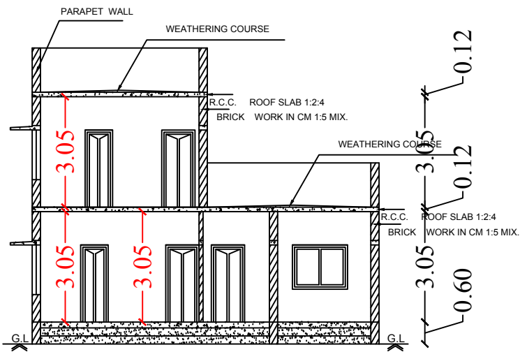
Section on-"AA"
