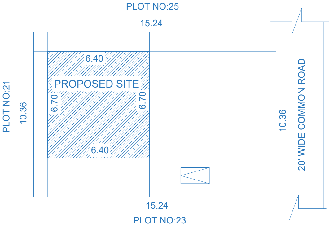
SITE PLAN
