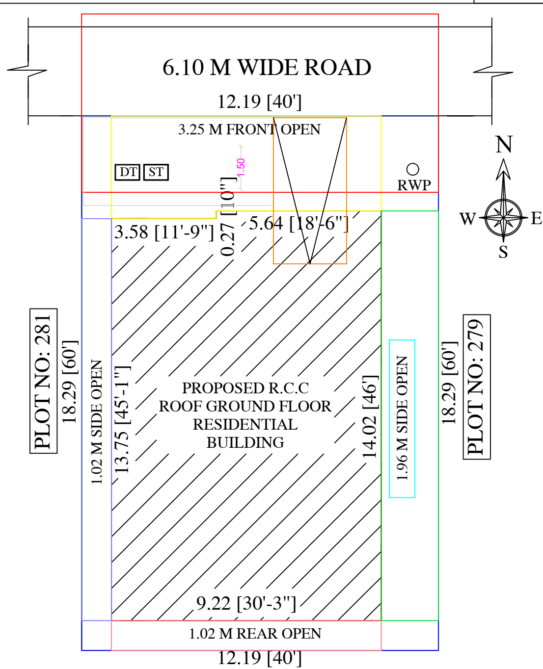
SITE PLAN
