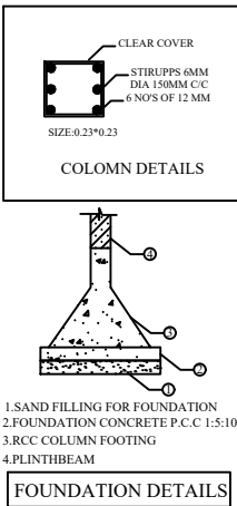
FOUNDATION DETAILS
