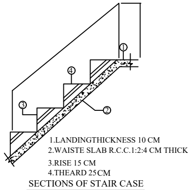
SECTIONS OF STAIR CASE
