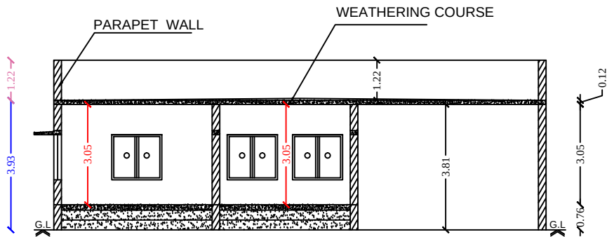
Section on-"AA"
