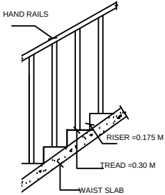
R CASE DETAILS
