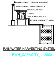
Section RR
