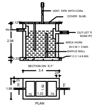
SEPTIC TANK DETAILS (NOT TO SCALE)
