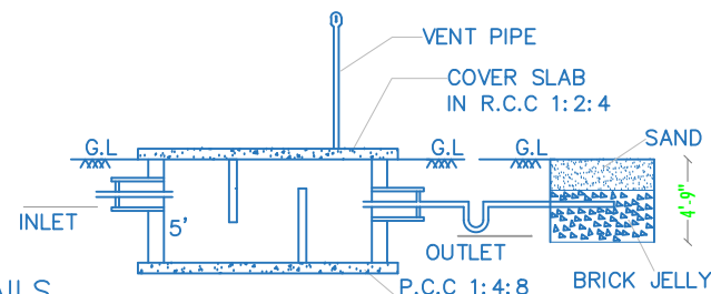
SECTION—AB
