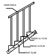
STAIR CASE DETAILS
