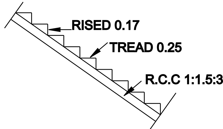
STAIRCASE DETAILS
