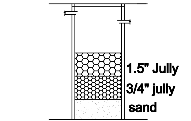
RAIN WATER HARVESTING TANK
