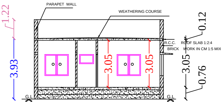
Section on-"AA"
