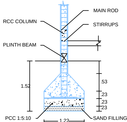
COLUMN DETAILS
