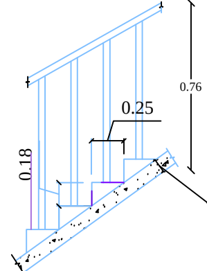
SECTION OF STAIRCASE
