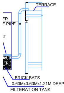
RAIN WATER HARVESTING SYSTEM
