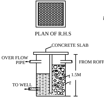
SECTIONS OF R.H.S.
