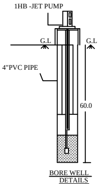
BORE WELL DETAILS
