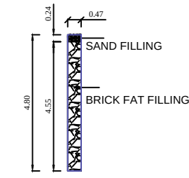
DETAILS OF PERCUSSION PIT
