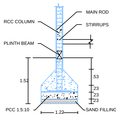
COLUMN DETAILS
