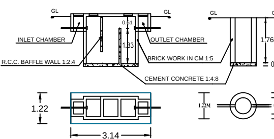
DETAILS OF SEPTIC TANK & SOAK PIT.
