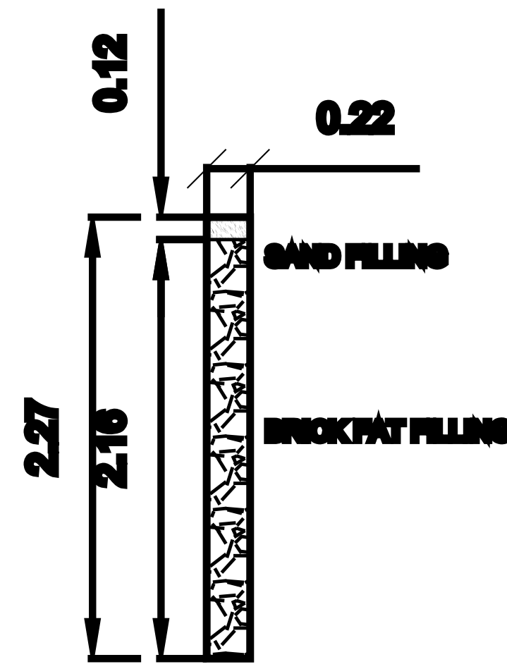
DETAILS OF PERCUSSION PIT
