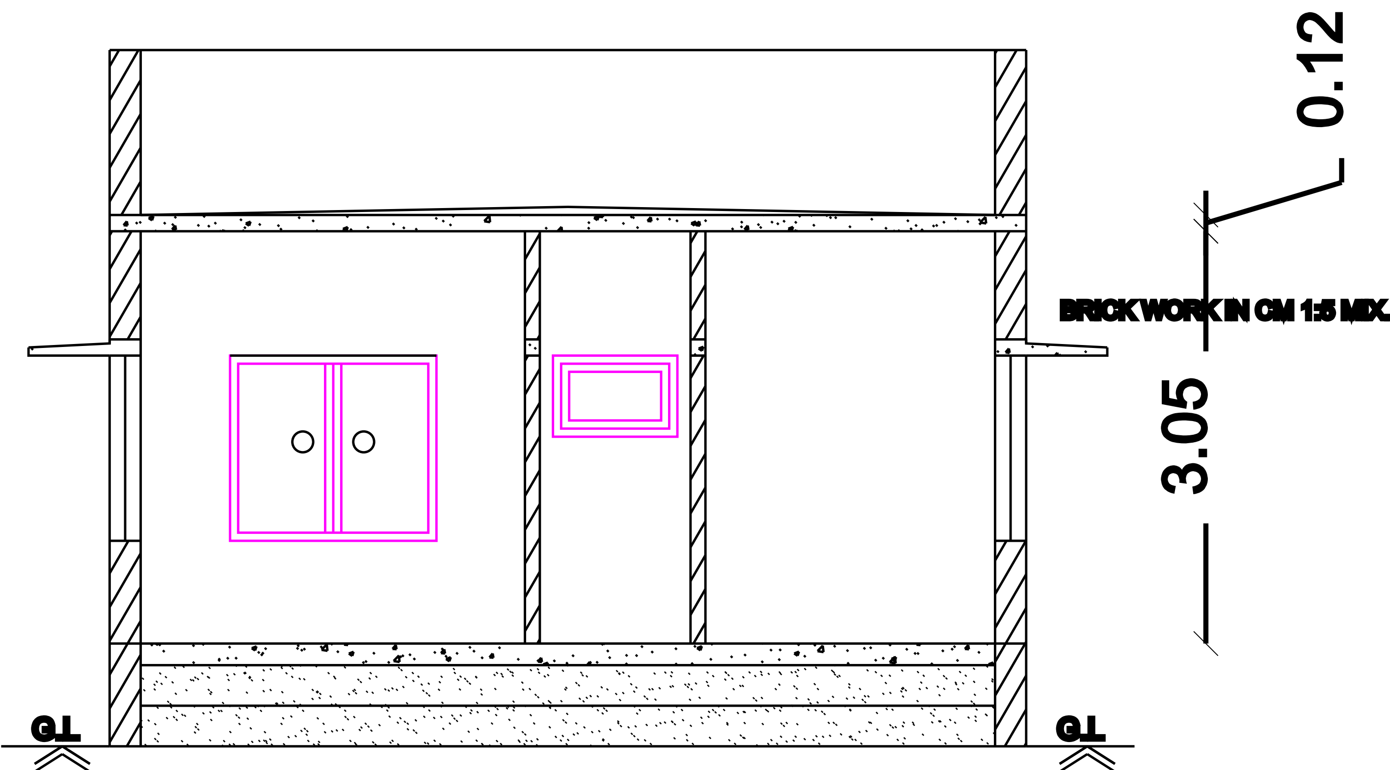
Section on-"AA"
