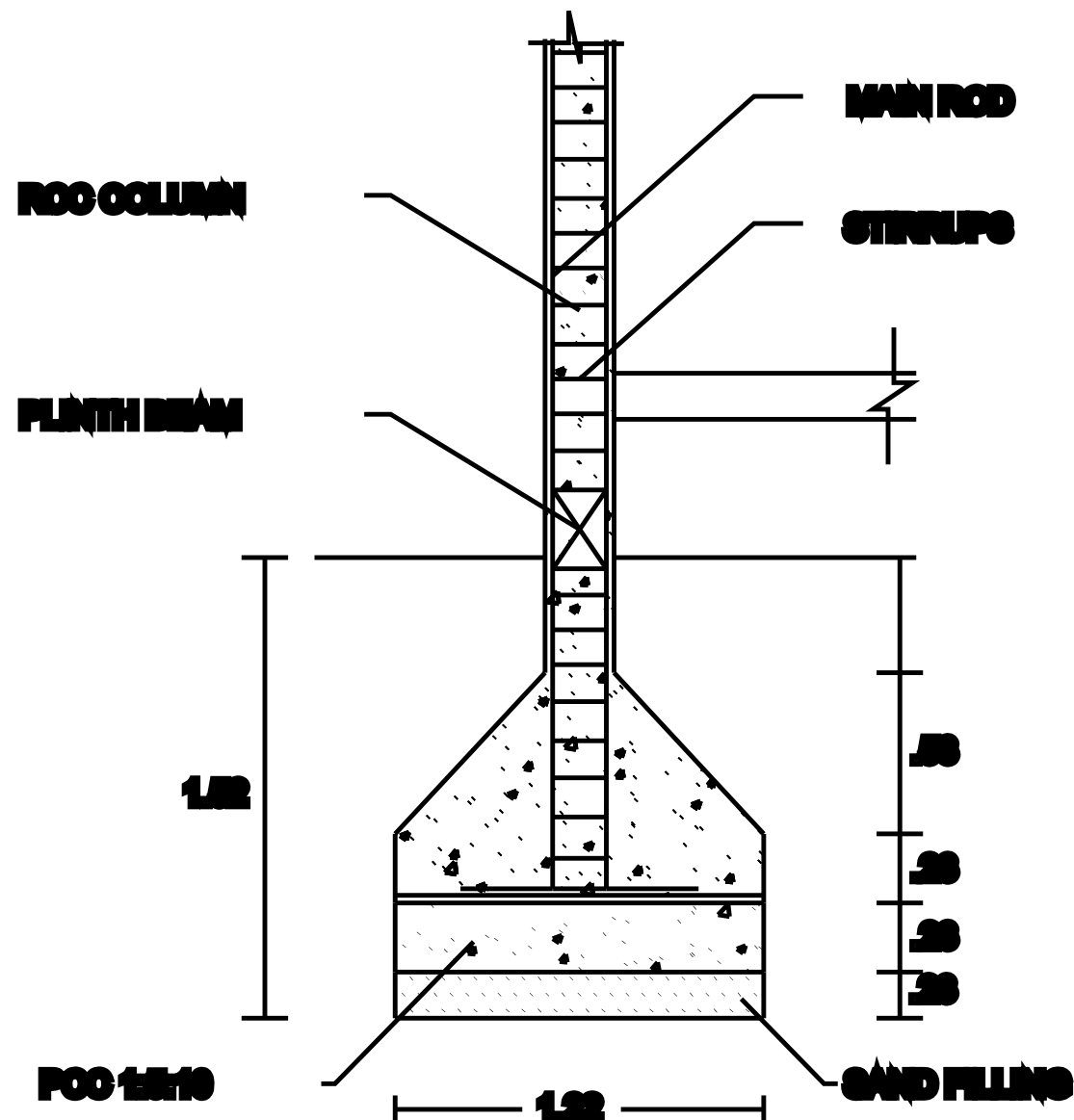
COLUMN DETAILS
