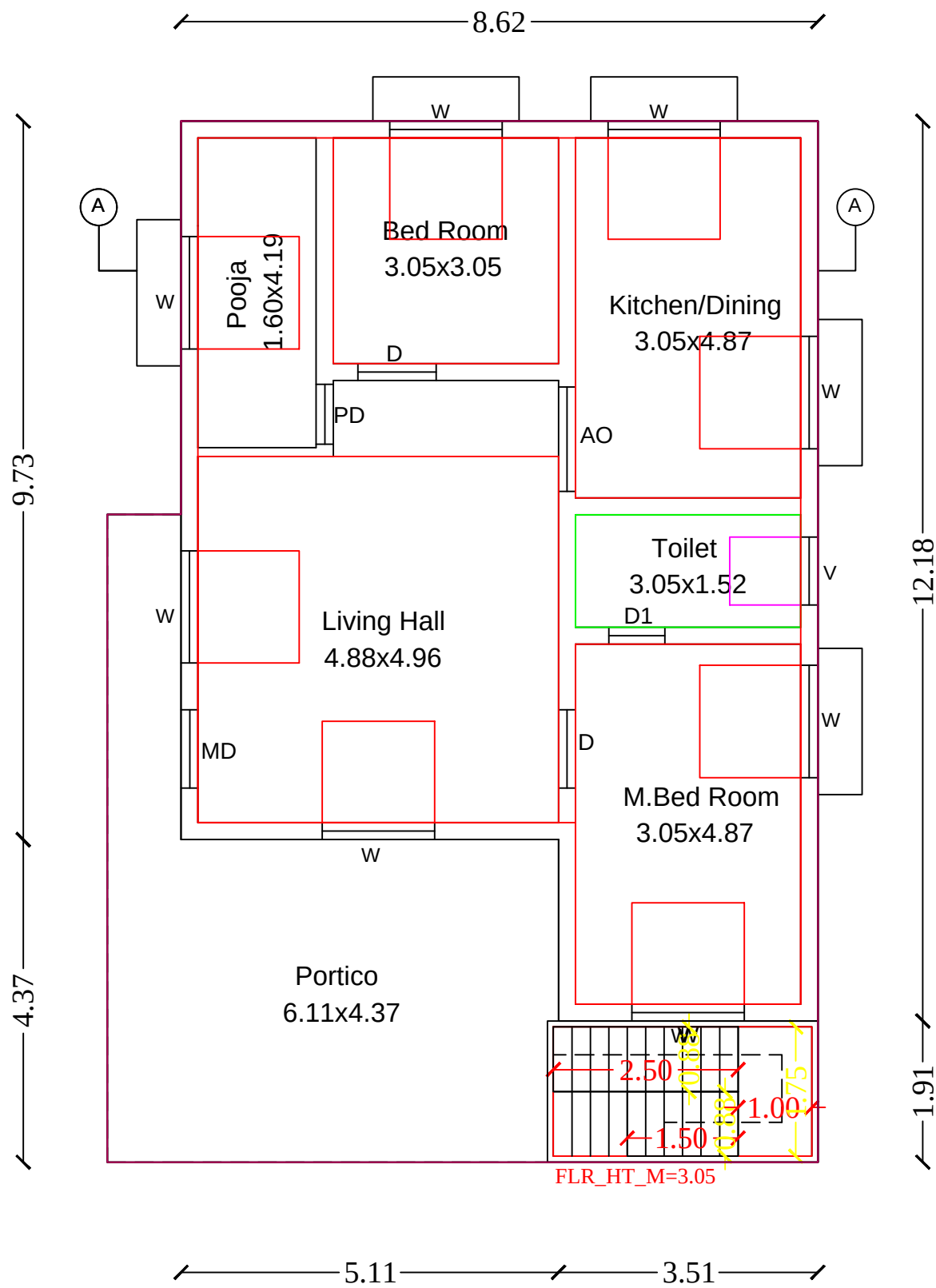
Ground Floor
