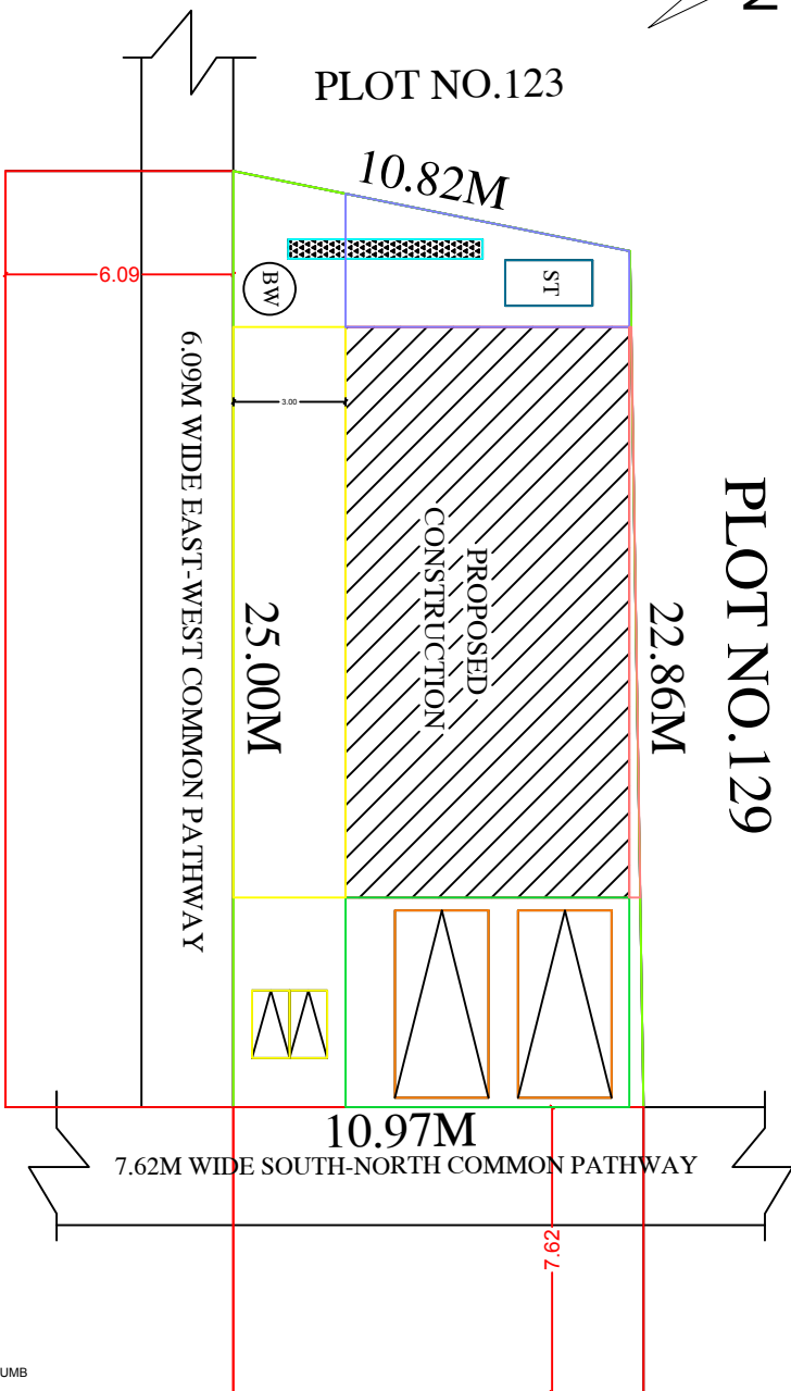
SITE PLAN
