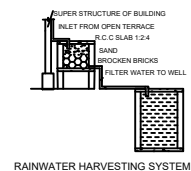
RAINWATER HARVESTING SYSTEM RWH_CAPACITY_L=2000
