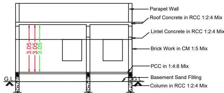
Section RR
