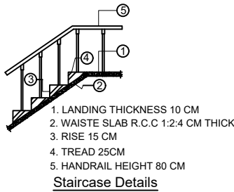
Staircase Details
