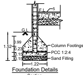
Foundation Details
