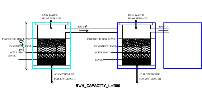
DETAILS OF PERCOLATION PIT
