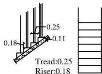
STAIRCASE DETAIL
