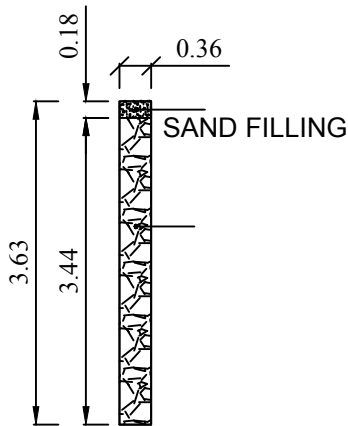
DETAILS OF PERCULATION PIT
