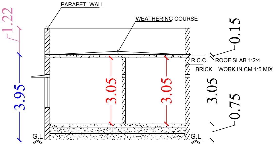
Section on-"AA"
