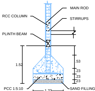
COLUMN DETAILS
