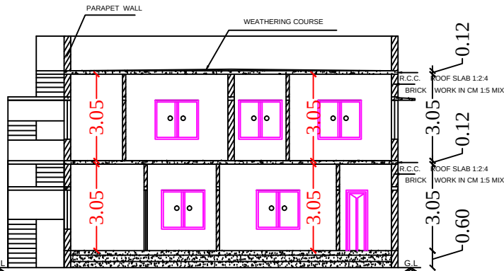
Section on-AA
