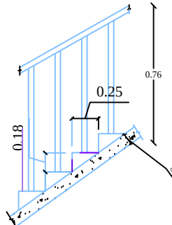
SECTION OF STAIRCASE
