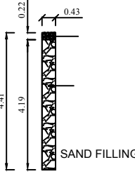
DETAILS OF PERCOLATION PIT
