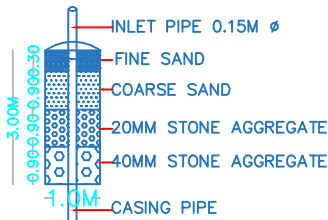
DETAILS OF RAIN WATER HARVESTING STRUCTURES
