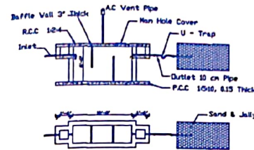
Septic Tank with Dispersion Trench
