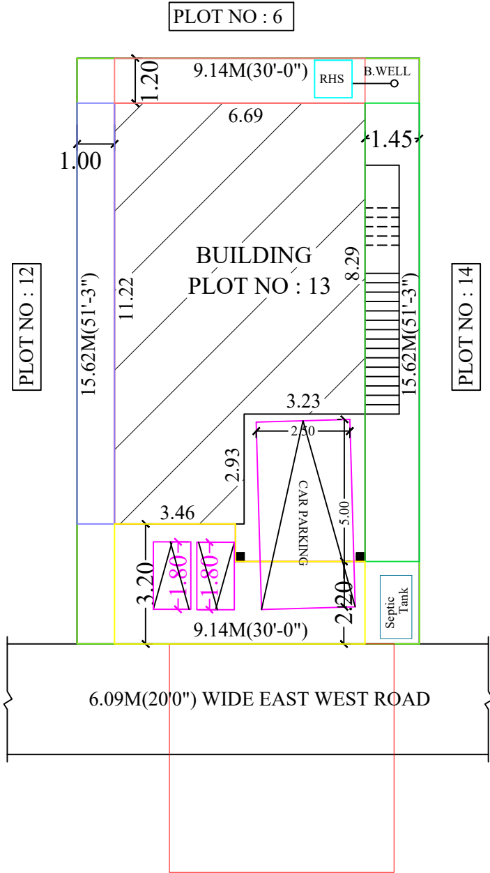
SITE PLAN (1:100)
