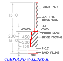
COMPOUND WALL DETAIL PLAN
