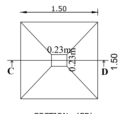
SECTION - 'CD'
