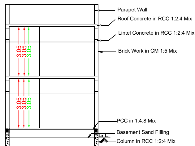
Section RR
