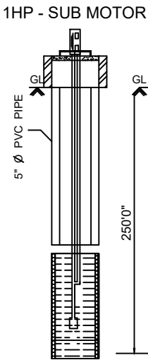
BOREWELL DETAILS
