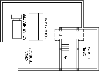
TERRACE PLAN
