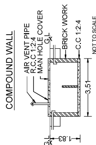
SEPTICTANK DETAILS
