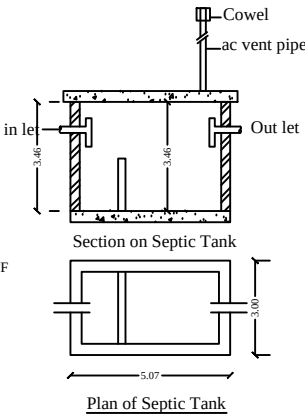
Plan of Septic Tank
