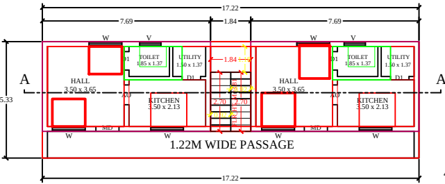
PROPOSED FIRST FLOOR
