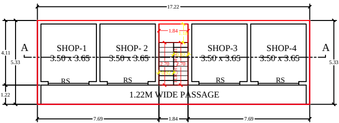
EXISTING GROUND FLOOR
