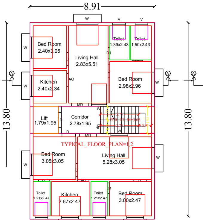
Typically First Floor & Second Floor
