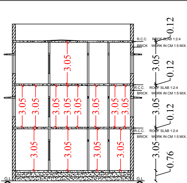
Section on-"AA"
