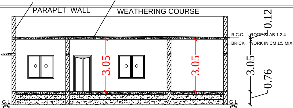
Section on-"AA"
