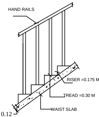
STAIR CASE DETAILS
