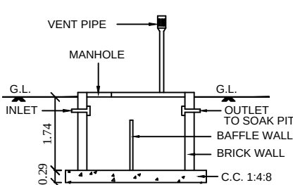
SECTION OF SEP. TANK
