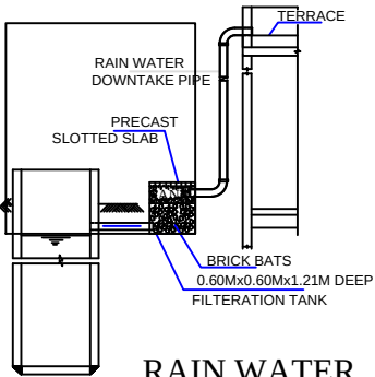
RAIN WATER HARVESTING SYSTEM
