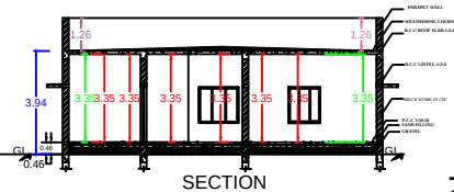
SECTION
