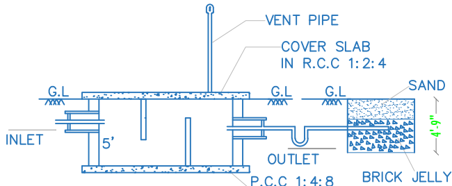
SECTION-AB
