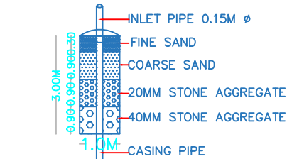
DETAILS OF RAIN WATER HARVESTING STRUCTURES
