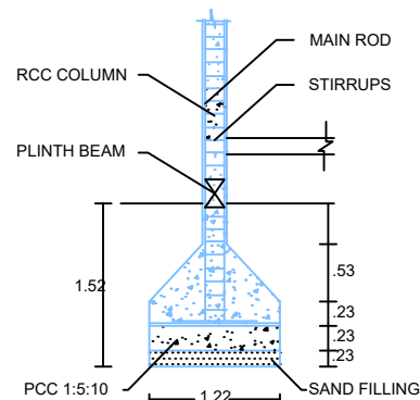
COLUMN DETAILS
