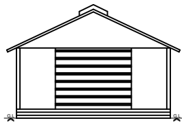
Front Elevation
