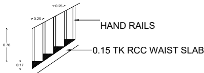
DETAILS OF STAIR CASE
