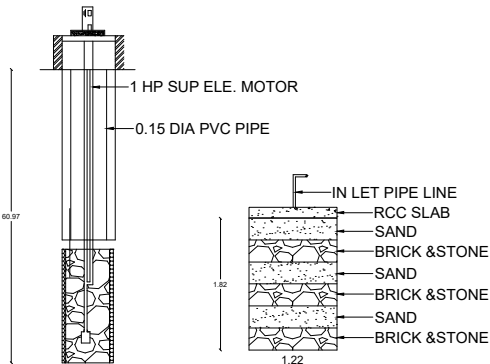
BORE WELL DETAILS
