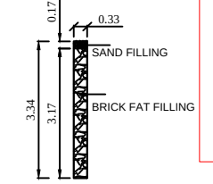
DETAILS OF PERCULATION PIT
