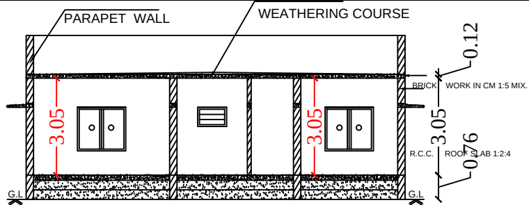
Section on-"AA"
