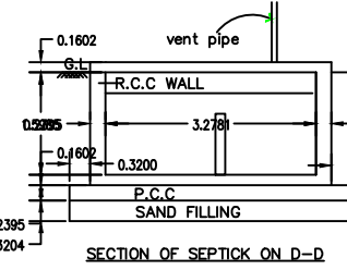
SECTION OF SEPTICK ON D-D
