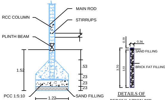
COLUMN DETAILS
