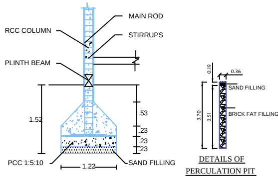
COLUMN DETAILS
