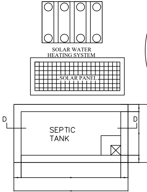
PLAN OF SEPTIC TANK SCALE 1"=2'0"
