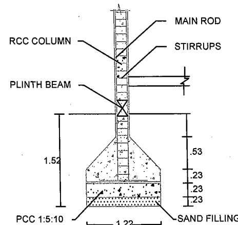
COLUMN DETAILS
